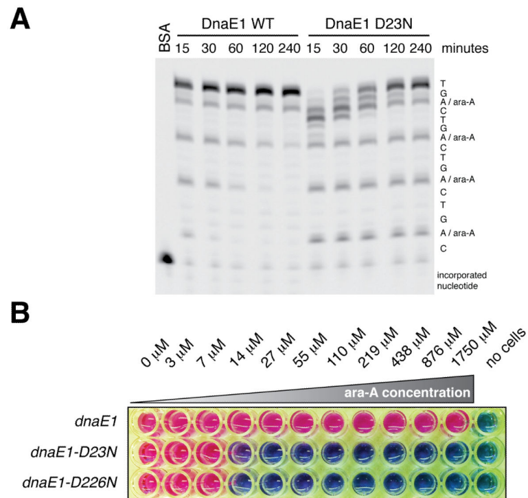
Figure 4. Inactivation of the PHP domain renders mycobacteria sensitive to nucleoside analogues (A) Primer extension analysis performed as in Figure 1H in the presence of 200 \mu\text{M} of the adenosine analog ara-A. Incorporation of ara-A impedes primer extension. Whereas wild-type DnaE1 MTB can excise ara-A and resume DNA synthesis, the PHP mutants cannot. (B) Determination of the minimum inhibitory concentration (MIC) of ara-A for the indicated M. smegmatis strains. Pink color indicates cellular respiration; blue color indicates lack of respiration.
