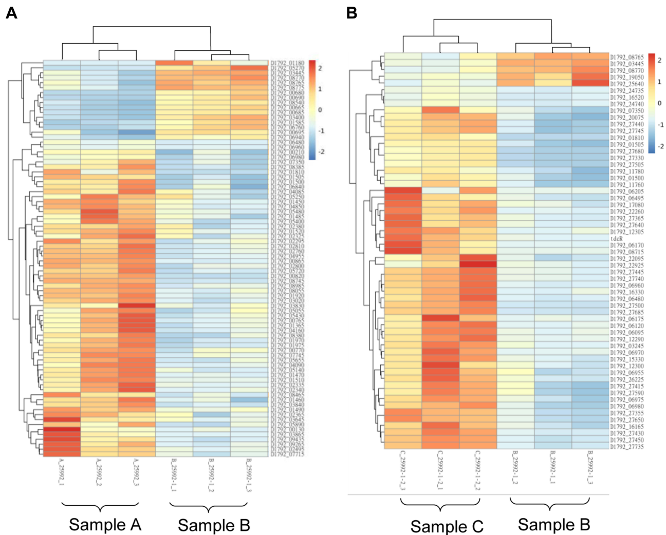
Figure 4 Heat map of hierarchical clustering in differentially expressed genes in the groups. (A) : E. coli ATCC 25922 (sample A) and E. coli ATCC 25922-R (sample B); (B) : E. coli ATCC 25922-R (sample B) and E. coli ATCC 25922-R grown with 2 mg/L colistin (sample C). Blue represents down-regulated expression and red represents up-regulated expression, respectively, relative to that of the reference culture.
