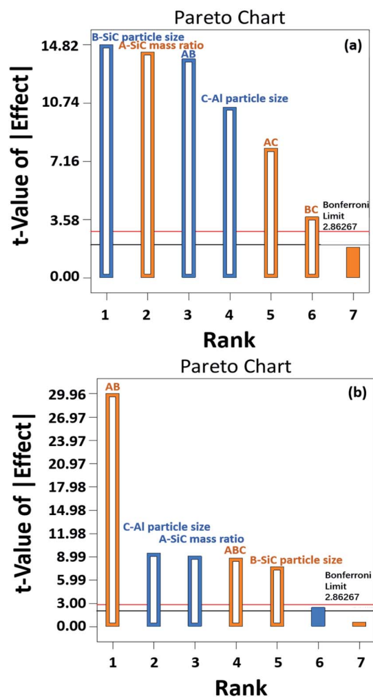
Fig. 5 Pareto chart of responses (a) S and (b) P .
