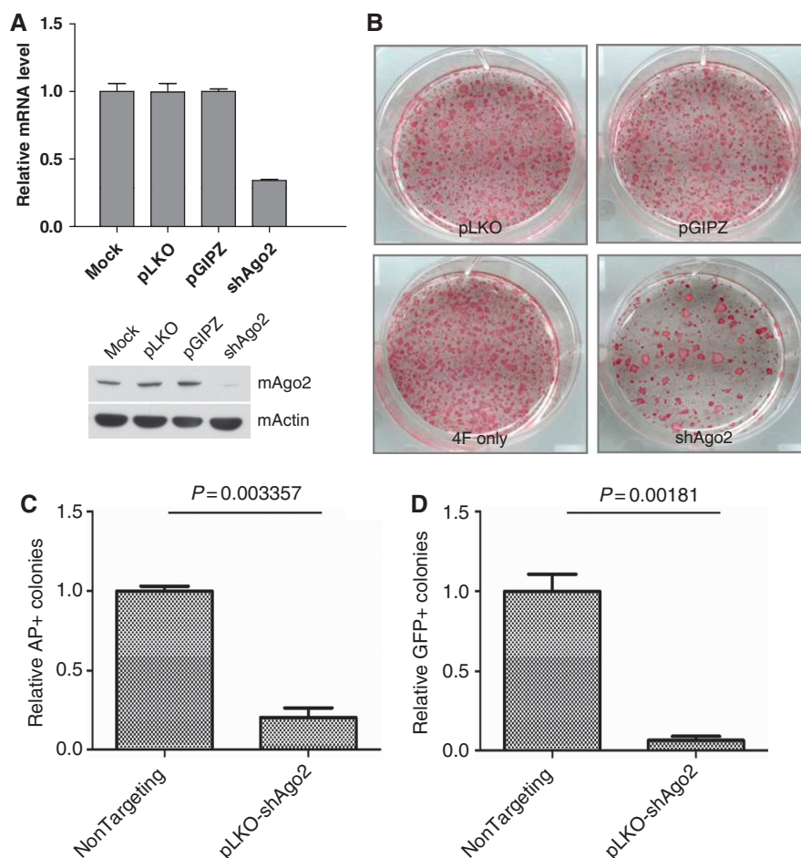
Figure 1 The RNAi machinery functions in mouse iPSC induction. (A) Knock-down of mouse RNAi machinery gene Ago2 by shRNAs. MEFs were transduced with lentiviral shRNAs plus 4 \mu g/ \mu l polybrene, and total RNAs or proteins were harvested at day 3 post-transduction. mRNA and protein levels of targeted genes were analysed by RT-qPCR and western blotting, respectively. pLKO is the empty vector control for the shRNA lentiviral vectors. pGIPZ is a lentiviral vector expressing a non-targeting shRNA. (B) Knock-down of Ago2 dramatically decreases iPSC induction by 4F. Primary MEFs were transduced with the four reprogramming factors (OSKM (4F)) plus shRNA Ago2. Colonies were stained at day 14 post-transduction for alkaline phosphatase (AP), which is a marker for mES/iPS cells. pLKO and pGIPZ vectors served as negative controls. (C) Knock-down of Ago2 decreases iPSC induction by OSK. Colonies were stained and quantified for AP at day 21 post-transduction. Error bar represents s.d. of duplicate wells. (D) GFP+ colony quantification of iPSC with shAgo2. GFP+ colonies were quantified at day 21 post-transduction. Error bar represents s.d. of duplicate wells.
