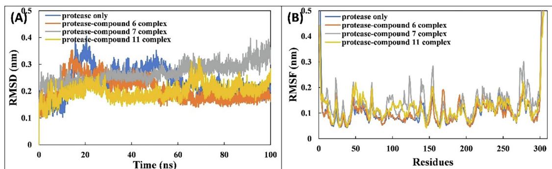
Fig. 2. (A) RMSD of the backbone of SARS-CoV-2 Mpro with compounds 6, 7, and 11 over 100 ns MD simulation. (B) RMSF of C_{\alpha} atoms of SARS-CoV-2 Mpro with compounds 6, 7, and 11.
