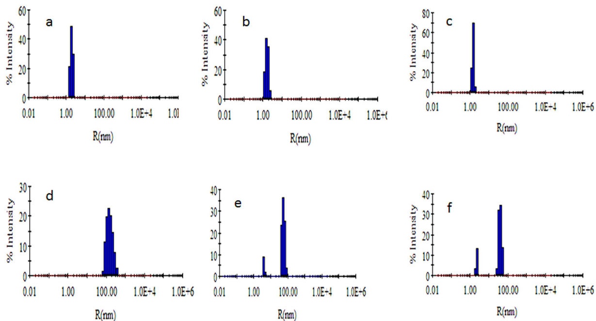
Figure 3. DLS pattern of HEWL in absence and presence of vitamin k3 at 25 °C (a) HEWL (b) HEWL + 50 \mu\text{M} vitamin k3 (c) HEWL + 100 \mu\text{M} vitamin k3 and after incubation at 65 °C over a period of 120 hours (d) HEWL (e) HEWL + 50 \mu\text{M} vitamin k3 and (f) HEWL + 100 \mu\text{M} vitamin k3.
