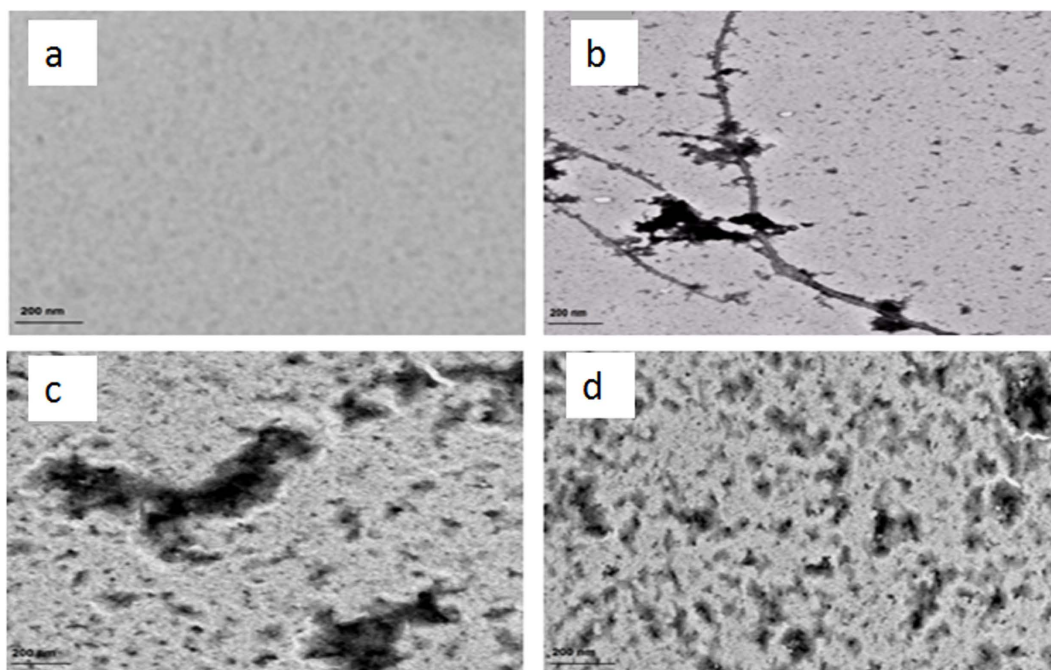
Figure 4. Transmission Electron Microscopic images (a) HEWL at 25 °C (b) HEWL incubated at 65 °C over 120 hours (c) HEWL + 50 \mu\text{M} vitamin k3 incubated at 65 °C over 120 hours (d) HEWL + 100 \mu\text{M} vitamin k3 incubated at 65 °C over 120 hours.
