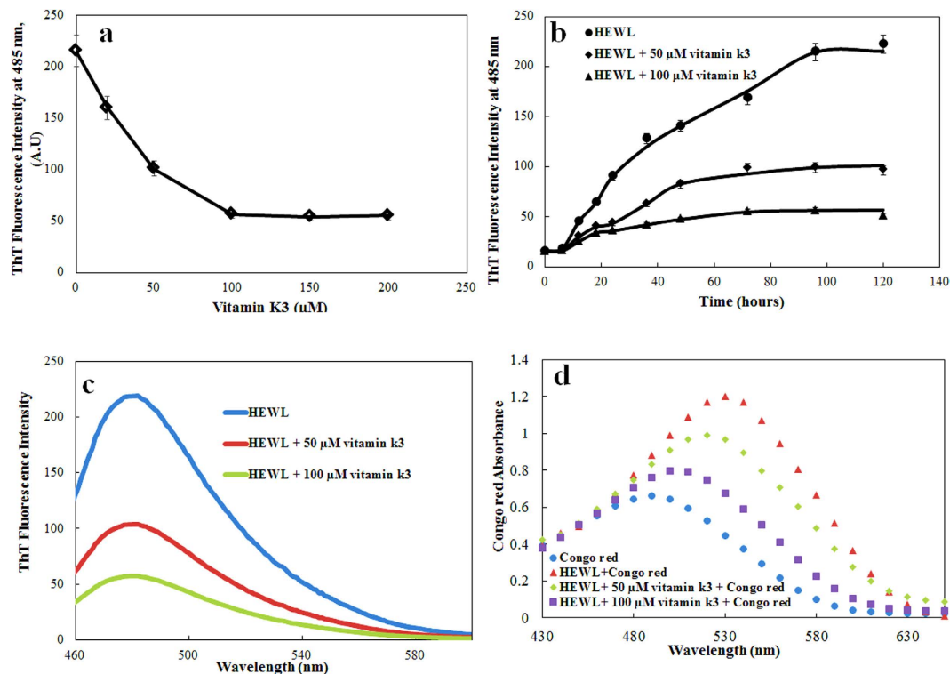
Figure 1. (a) ThT fluorescence intensity of HEWL (15 \mu\text{M} ) at 485 nm in presence of varying concentration of vitamin k3 (0–200 \mu\text{M} ). Samples were incubated at 65 ^{\circ}\text{C} for 120 hours. (b) ThT fluorescence kinetics of HEWL in absence and presence of vitamin k3 (50 and 100 \mu\text{M} ) (c) ThT fluorescence spectra of HEWL incubated at 65 ^{\circ}\text{C} over 120 hours in absence and presence of vitamin k3 (50 and 100 \mu\text{M} ) (d) Congo red binding absorption spectra of HEWL (15 \mu\text{M} ) in the absence and presence of vitamin k3. Samples were incubated with two different concentration of vitamin k3 (50 and 100 \mu\text{M} ) at 65 ^{\circ}\text{C} for 120 hours. Experimental data represent the average \pm s.d (n = 3).
