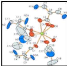
Fig. 1. ORTEP view of the asymmetric unit of (I) with thermal ellipsoids at 50% probability. Hydrogen atoms are omitted for clarity.
