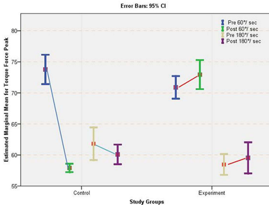
Figure 8 The differences in torque force peak between groups in interaction with time and angle.
