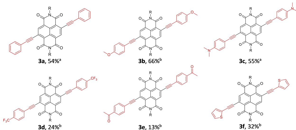
Figure 4. Scope of c-NDI synthesised by Sonogashira coupling ( 3a–3f ) using VBM and isolated by flash column chromatography. Isolated yields after flash column chromatography reported. [a] Using precatalyst Pd(OAc) 2 , [b] using precatalyst C2 ; R = 2-ethyl hexyl chain.
