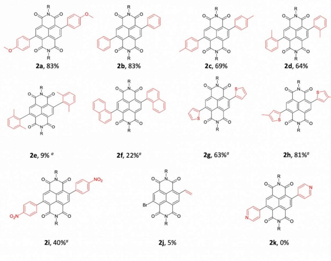
Figure 2. Scope of c-NDI products 2a–2k synthesised by Suzuki coupling using VBM methods and isolated by flash column chromatography. Isolated yields. [a] Cycloocta-1,5-diene (10 wt%) as LAG agent. R = 2-ethylhexyl chain.
