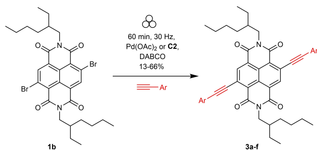
Scheme 2. Synthesis of Sonogashira c-NDIs.
