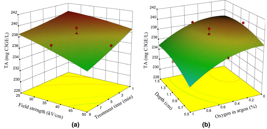
FIGURE 6 (a) The effect of field intensity and plasma exposure time, and (b) the effect of samples depth and oxygen content in argon on TAC in sour cherry juice
