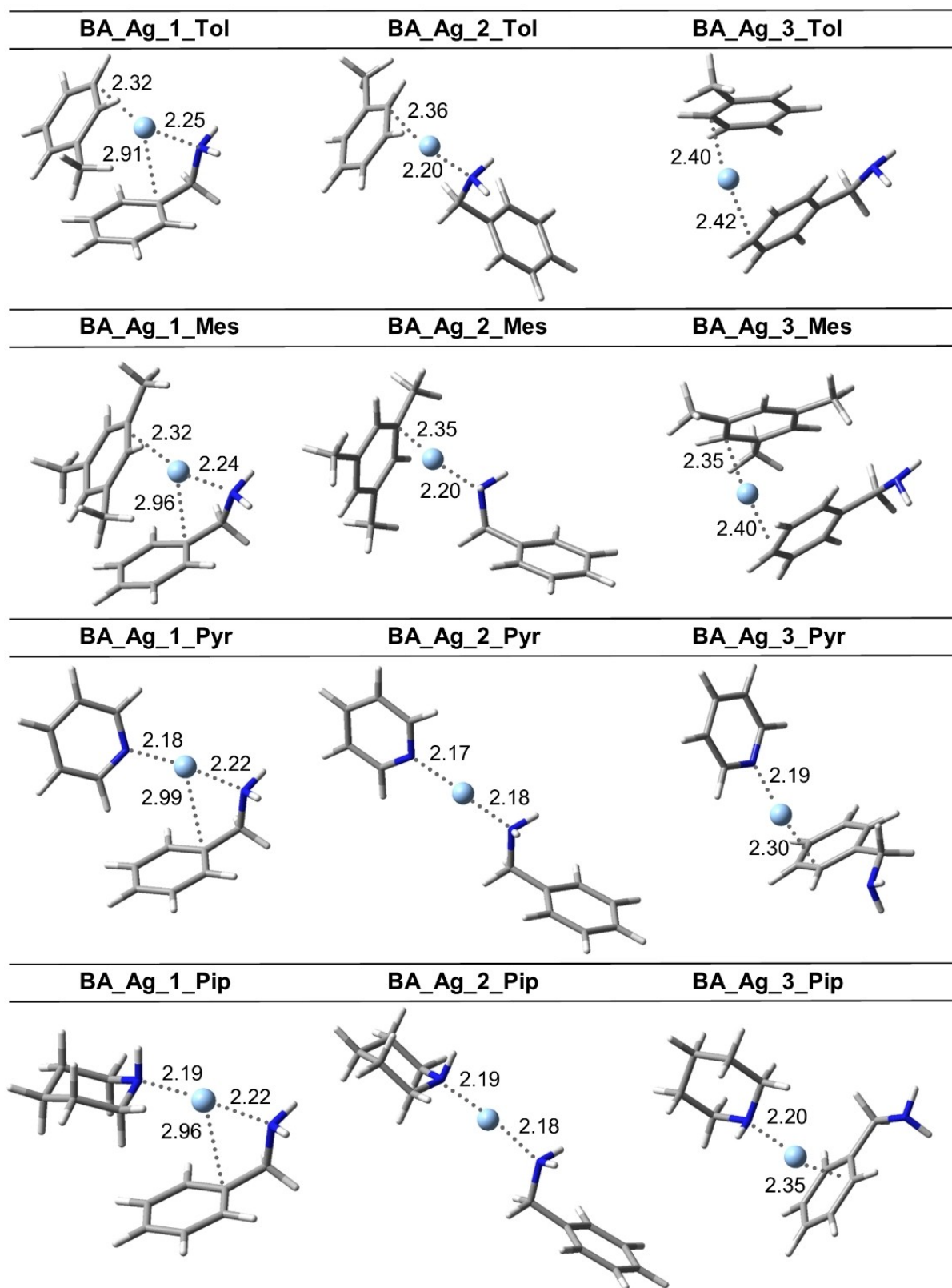
Figure 4. Optimized geometries for \text{Ag}^+(\text{BA})(\text{L}) ions (L = Tol, Mes, Pyr, Pip) at the MP2 level. Bond distances (in Å) are indicated by dashed lines.
