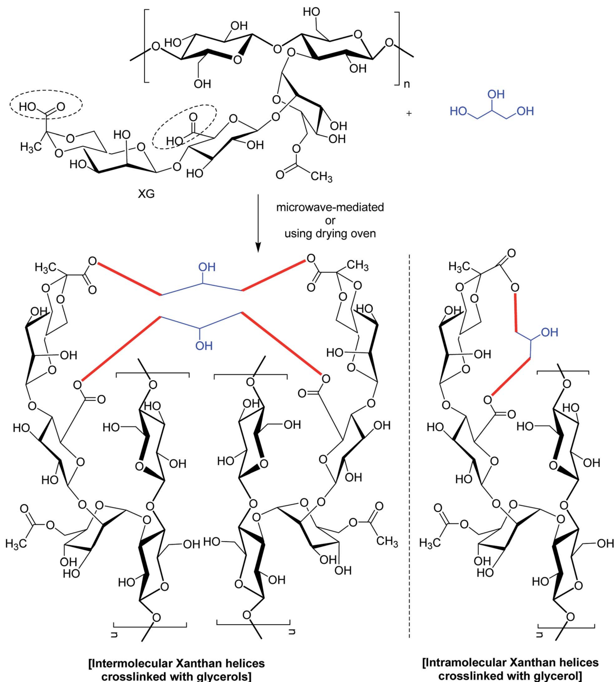
Fig. 8 Glycerol-crosslinked XG.
