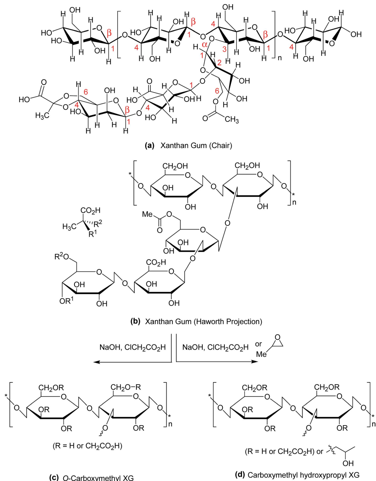
Fig. 1 Chemical structure of (a) XG (chair conformation); (b) XG (Haworth projection); (c) carboxymethyl XG; (d) carboxymethyl hydroxypropyl XG.
