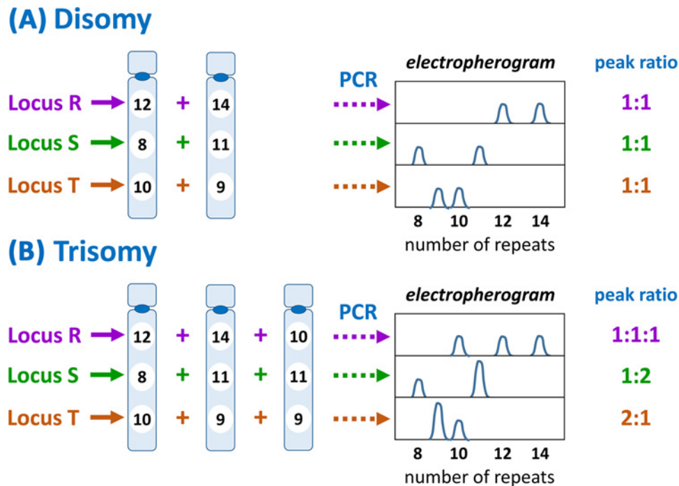
Figure 43. QF-PCR
