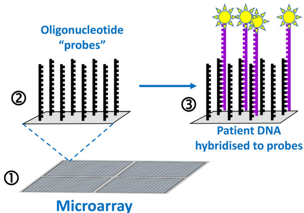
Figure 45. Basic microarray
