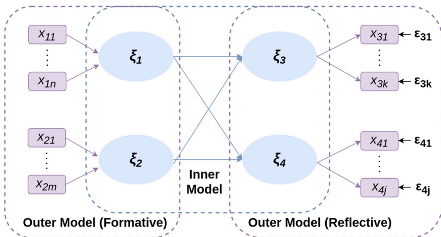
Fig. 1 Path model definition
