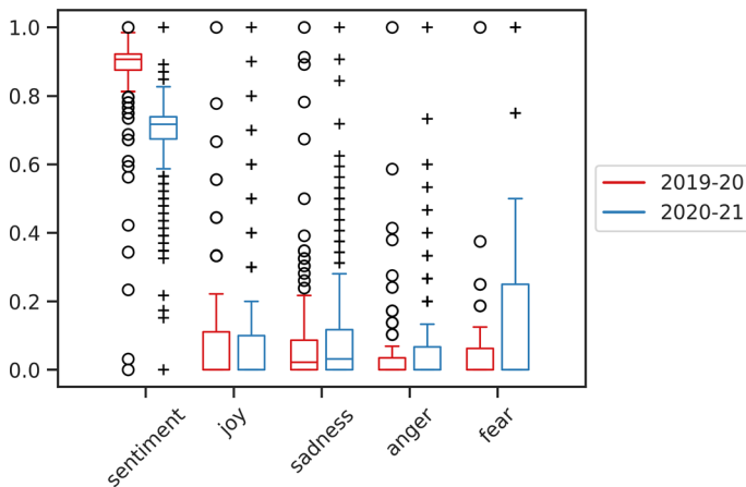
Fig. 4 Normalized version of Sentiment \mathcal{F}_{\text{Sen}} and the four emotions in the two academic years analyzed
