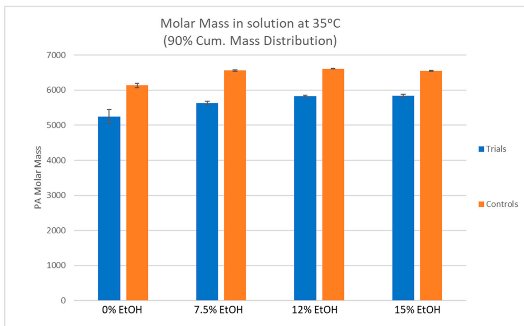
Figure 3. The results of gel permeation chromatography (GPC) analysis comparing molar mass (at 90% cumulative mass distribution) of trial and control solutions at the end of the desorption experiments (samples taken at 35 °C).
