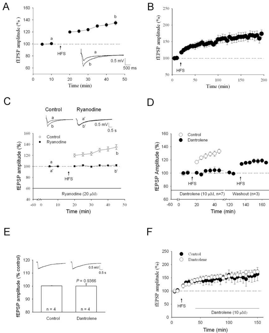
Figure 1 Involvement of RyR in the induction of LTP of fEPSPs in the spinal dorsal horn in vitro . A , fEPSPs were recorded in the presence of 10 \mu M bicuculline methiodide and 1 \mu M strychnine. fEPSPs recorded 10 min before HFS served as control. After HFS, fEPSPs significantly increased ( n = 24 ). The inserted traces were the original recordings (without averaging). a-b corresponds to the time points as indicated. B , The LTP of fEPSPs stably lasted for 3 h ( n = 8 ). C , 20 \mu M ryanodine applied 1 h before HFS blocked the induction of LTP ( P < 0.001 ) (control n = 7 ; ryanodine n = 8 ). The inserted traces were the original recordings. D , 10 \mu M dantrolene perfused 1 h before HFS blocked the induction of LTP ( P < 0.001 ) (control n = 7 ; dantrolene n = 7 ), and this effect was reversible ( P < 0.001 ) (washout n = 3 ). E , 10 mM dantrolene has no significant effect on the amplitude of fEPSP. Control: the amplitude of fEPSP recorded 5 min before dantrolene application (10 \mu M); Dantrolene: 30 min after perfusion of dantrolene. Inserts show original traces recorded 5 min before and 30 min after dantrolene. F , 10 \mu M dantrolene perfused 30 min after HFS had no significant effect on the established LTP ( P = 1 ) (control n = 5 ; dantrolene n = 6 ). Data were shown as mean \pm s.e.m. in all figures; n : the number of slices.
