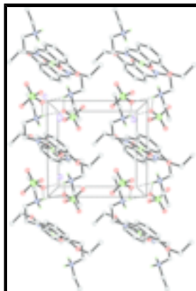
Fig. 2. The crystal packing of (I), viewed along the c axis.
