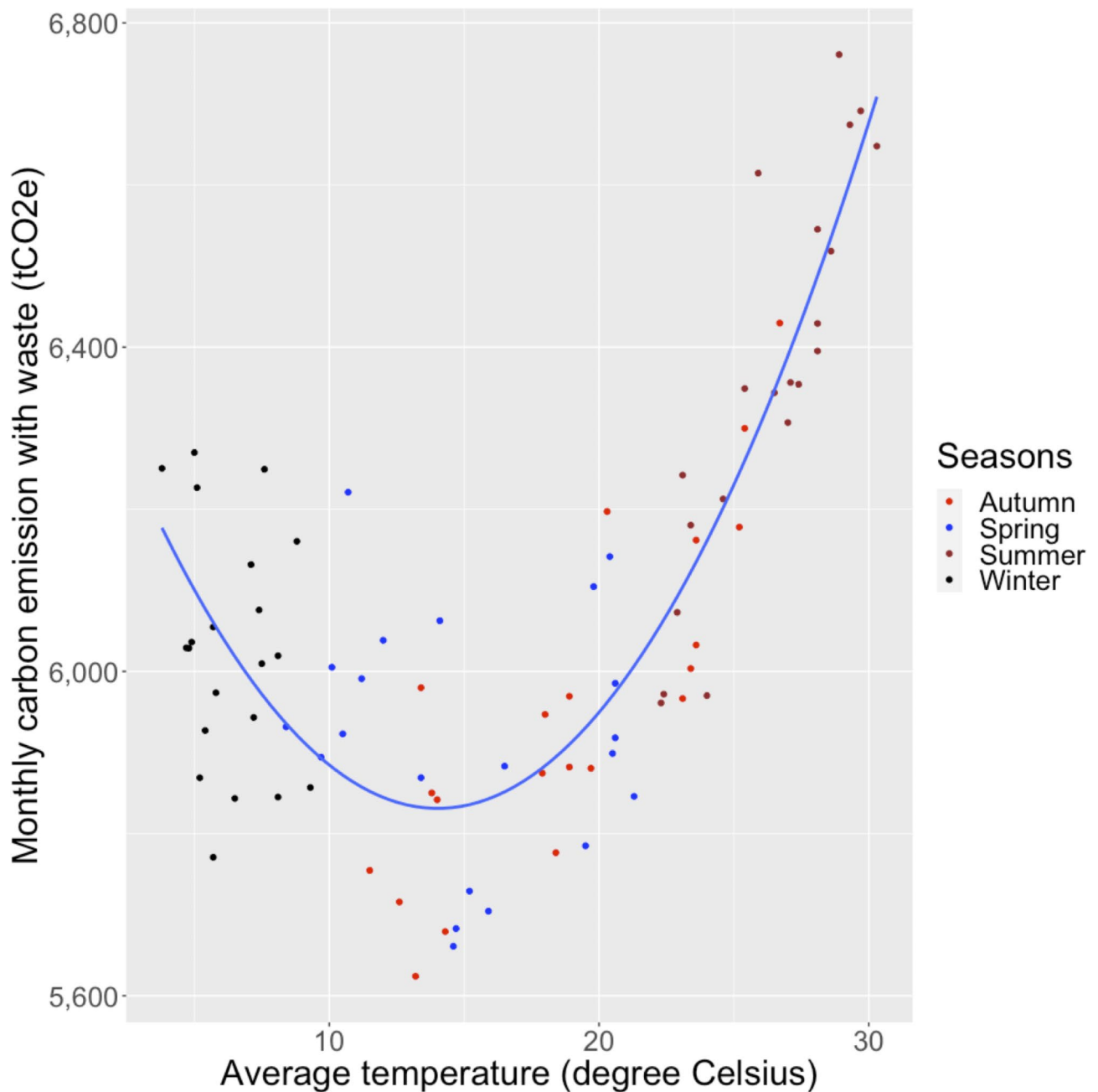
Fig. 3 Correlation between monthly average external temperature and monthly carbon footprint from April 2014 to March 2021. Autumn: September, October, November. Spring: March, April, May. Summer: June, July, August. Winter: December, January, February
