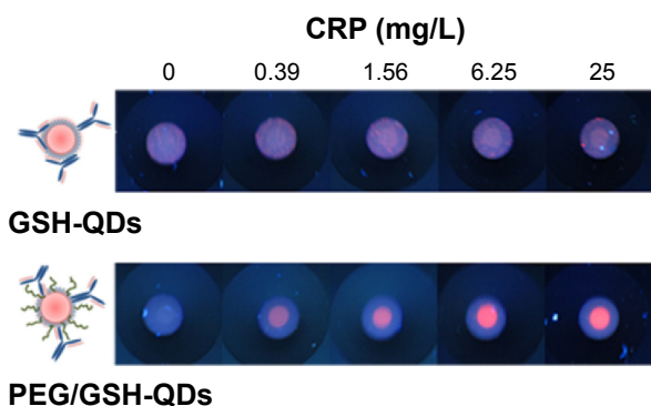
Figure 3 Comparative detection of CRP using QDs labeling conjugates prepared from GSH-QDs and PEG/GSH-QDs conjugates.
