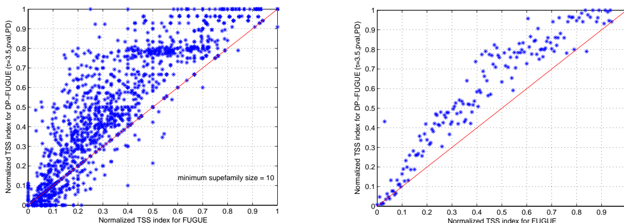
Figure 5 Comparison of the normalized TSS index of FUGUE and DP-FUGUE. Left: Scatter plot based on all queries in the test set that belong to SCOP superfamilies containing at least 10 members. Right: Averaged scatter plot (for each TSS value of FUGUE we average all TSS indices of DP-FUGUE that are associated with that value). Points situated above the diagonal represent successful cases where the TSS index is improved when using the DP representation and vice versa.
