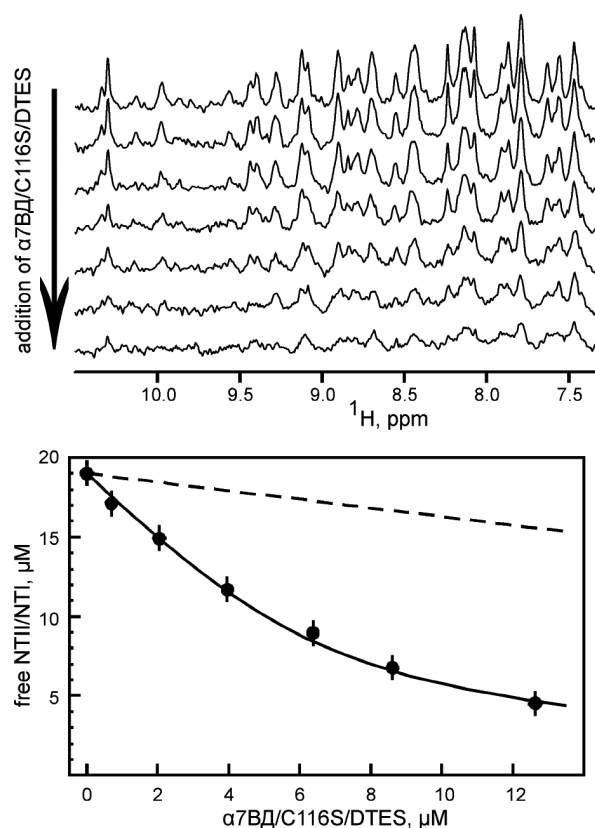
Fig. 4. 1D ^{15}N -HSQC NMR spectrum of NTII/I toxin in the presence of DPC micelles and following an increase in \alpha 7BD/C116S/DTES concentrations. The obtained isotherm binding and dilution curves (dashed line) are shown.
