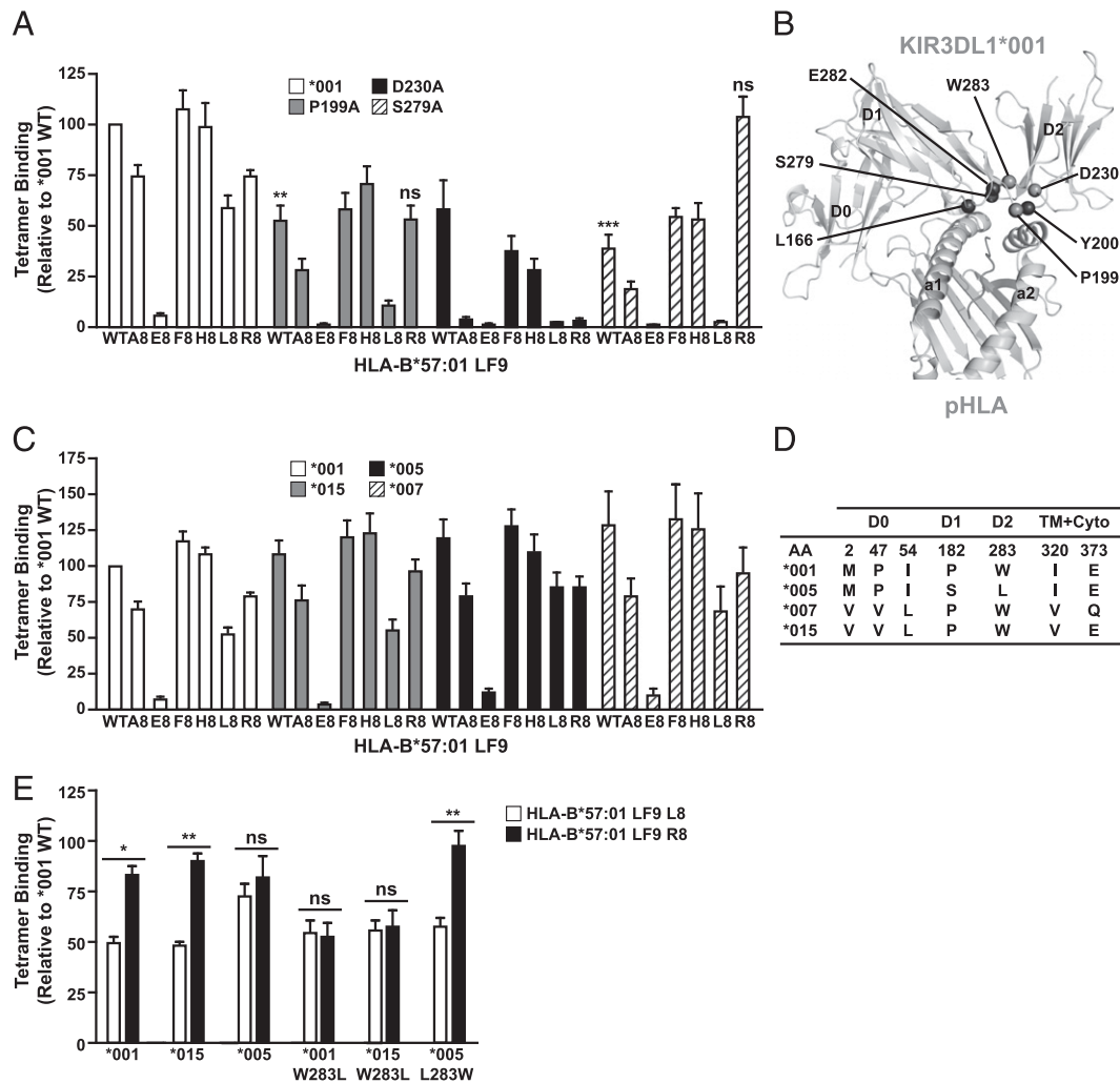
FIGURE 2. Allotypic variation influences peptide preference. ( A , C , and E ) HEK293 cells were transfected with FLAG-tagged 3DL1*001, other 3DL1 allotypes, or mutants thereof and stained with individual HLA-B*57:01-LF9 tetramers (0.2 \mu g each) as indicated. Data are averaged from at least n = 3 independent experiments. * p < 0.05 , ** p < 0.01 . Statistical significance relative to 3DL1*001 binding was assessed by ANOVA with a Tukey multiple comparison posttest. Error bars represent SEM. ( B ) The structure of 3DL1*001-HLA-B*57:01-LF9 with residues of interest highlighted. ( D ) Alignment of the 3DL1 allotypes used in this study. Variable residues are numbered and grouped by protein domain in the mature full-length protein.
