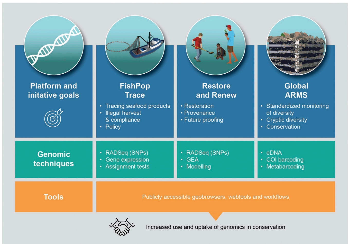
Fig 2. Tools, techniques, and platforms for using genomic data in marine conservation. Examples of applied online tools and platforms that assist biodiversity managers and conservation practitioners in the use genomic data. GEA; genotype-environment associations.
