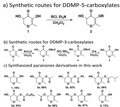
Scheme 1 Synthetic routes for DDMP derivatives.
