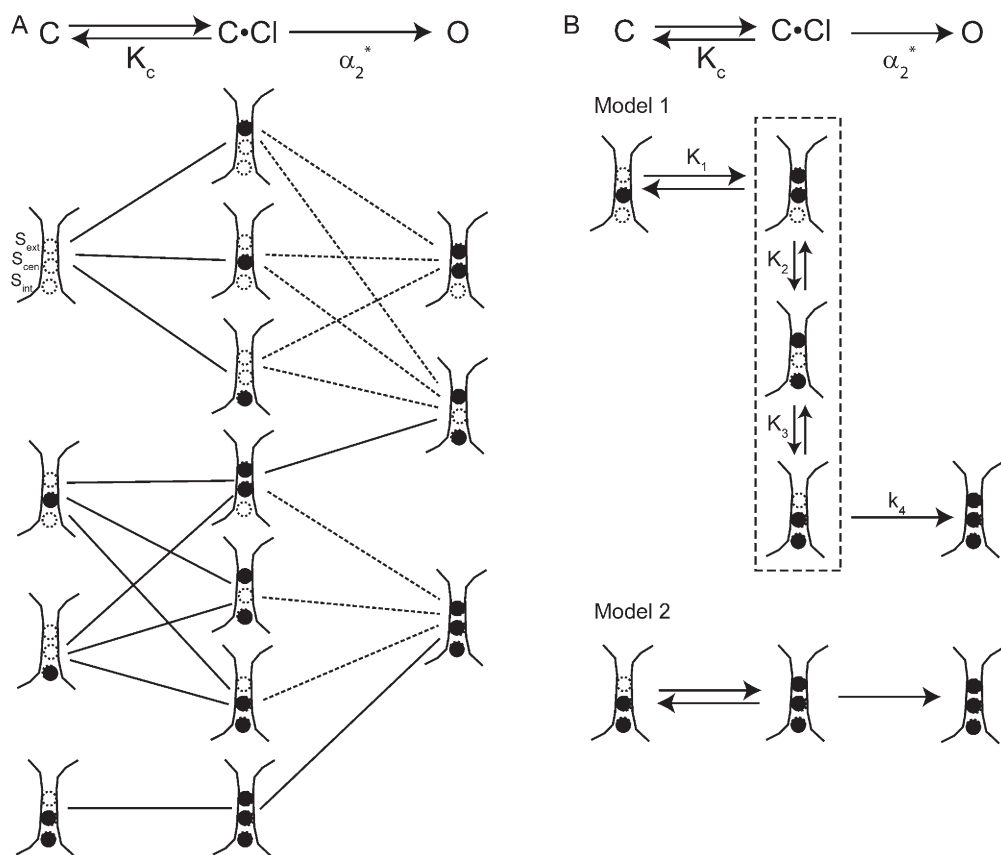
Figure 7. Possible models for chloride movement during depolarization-activated fast gating. Evidence from previously published papers and our kinetic and homology model analysis was used to narrow down the possible models for chloride movement during depolarization-activated fast-gate opening to those shown (see text). The channel begins in the closed state C, binds chloride to reach the closed state C·Cl, and then goes through another depolarization-activated transition to reach the open state O. This is depicted at the top of both A and B. K_c is the apparent equilibrium constant for chloride dissociation, and \alpha_2^* is the rate constant for the second step, C·Cl→O. In A, depicted below each of these states (C, C·Cl, and O) are their possible chloride occupancy states, with empty circles depicting vacant chloride binding sites, and filled circles depicting filled chloride binding sites. Lines between these chloride-occupancy states indicate transitions
