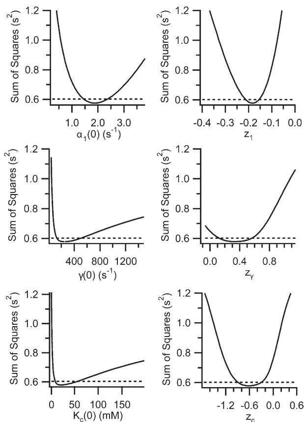
Figure 4. Error analysis on fits to the five-state model. To determine the certainty of the best-fit values found when globally fitting \alpha(V, [Cl]_{ext}) to the five-state model (Method 2), we used the procedure described in the text. Each of the plots shows how varying one of the six parameters affects the goodness of fit to our data as given by the sum of squares (solid lines). The sum of squares at 95% confidence is shown as a dashed line, and the parameter values at the intersections of the solid line and dashed line represent the 95% confidence limits, shown as error bars in Fig. 5. A similar procedure was used to calculate the 95% confidence limits on the four-state model parameter values, which are shown as error bars in Fig. 3, columns 6 and 7 of each graph.
