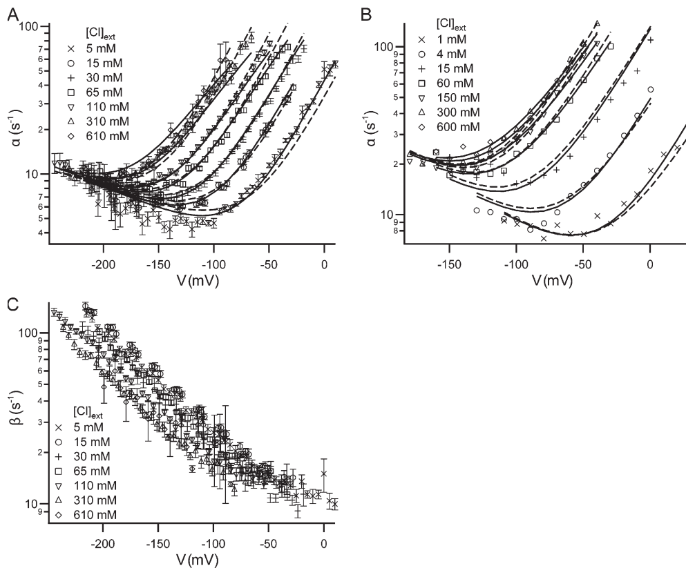
Figure 2. Effect of voltage and external chloride on the kinetics of fast gating. (A and C) opening ( \alpha ) and closing ( \beta ) rate constants for each test voltage. For test pulses (see examples in Fig. 1 A) where current decay could be seen, the decay was fit to a single exponential to derive the decay constant ( 1/\tau ). This was used in conjunction with the open probability ( P_o ) to calculate \alpha and \beta (Chen and Chen, 2001): \alpha = P_o/\tau ; \beta = (1/\tau) - \alpha . For each condition (voltage (V), external chloride activity ( [Cl]_{ext} ), we recorded from at least five patches and derived the rate constant for each patch. For the 610 mM chloride condition, we recorded two to five patches for each voltage. For a given condition, the rate constants from all patches were averaged; the error bars show the SEM. (B) For comparison, opening rate constant data were taken from the graphs published by Chen and Miller (1996) and replotted.
