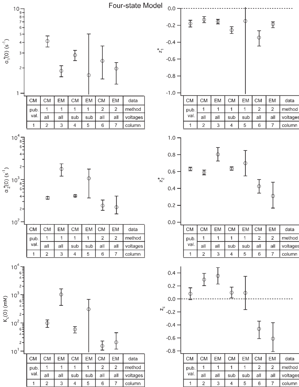
Figure 3. Parameter values for the four-state gating model. Values for the four-state model parameters were derived for both the dataset published by Chen and Miller in 1996 (CM) and for the dataset we obtained using macroscopic recordings (EM). These parameter values were derived using two different fitting methods: (1) Method 1, used by Chen and Miller, shown in Figure S4; and (2) Method 2, globally fitting the opening rate constant as a function of voltage and external chloride ( \alpha(V, [Cl]_{ext}) ), allowing all six parameters to be free, shown as solid lines in Fig. S5, C and F. Method 1 was performed including either all the voltages (all) or some subset of the voltages (sub). For Method 1, the error bars show the standard deviation calculated by the fitting algorithm (for fits shown in Fig. S4, B and D); for Method 2, the error bars show the 95% confidence limits determined as described in the text. For comparison, the parameter values ( z_1^* , z_2^* , and z_c ) published by Chen and Miller (pub. val.); values for \alpha_1^*(0) , \alpha_2^*(0) , and K_c(0) were not reported.
