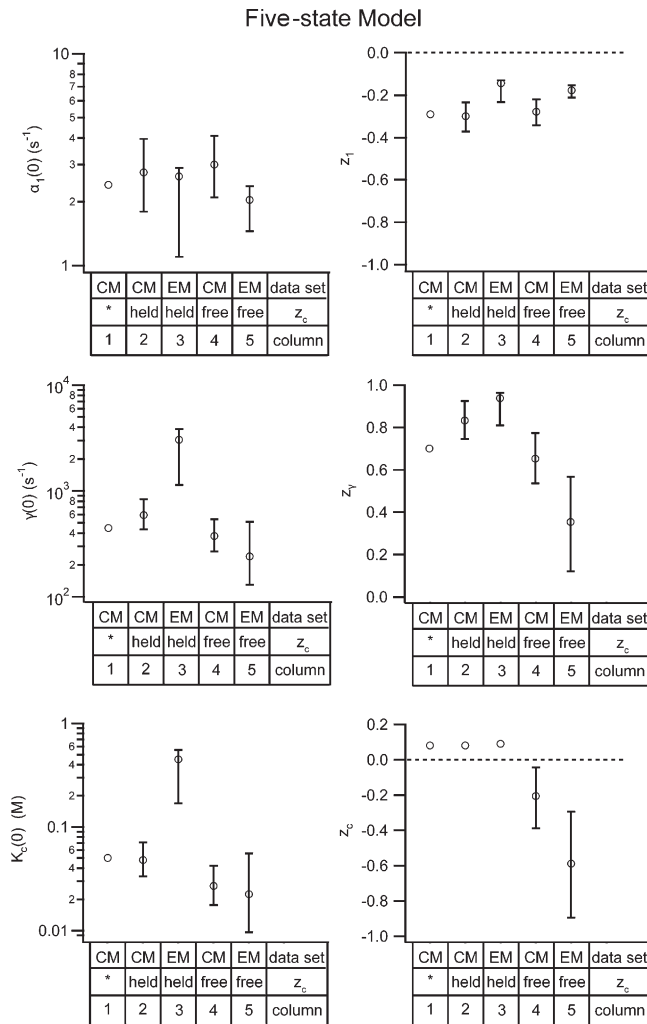
Figure 5. Parameter values for the five-state gating model. Values for the five-state model parameters were derived for both the dataset published by Chen and Miller in 1996 (CM) and for the dataset we obtained using macroscopic recordings (EM). In both cases, parameter values were derived by globally fitting the opening rate constant as a function of voltage and external chloride ( \alpha(V, [Cl]_{ext}) ) (Method 2) (fits shown in Fig. 2, A and B), either with all six parameters free (free) or while holding z_c at 0.08 (held) (see the supplemental material for explanation, and Figs. 3 and S4, subset of voltages). The error bars show the 95% confidence limits determined as described in the text. For comparison, the first column shows the parameter values published by Chen and Miller (*).
