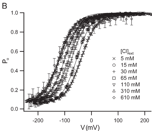
Figure 1. Effects of external chloride on gating. (A) Voltage pulse protocol (top left) and current responses in 5, 110, and 310 mM external chloride. (B) Tail-current analysis was used to determine the apparent open probability ( P_o ) as a function of voltage ( V ) (see Materials and methods) ( n = 5 –26 for external chloride concentrations <600 mM, and n = 2 –5 for 610 mM). These plots were fit as described in Materials and methods (solid lines), and gating parameters were derived (Table II).
