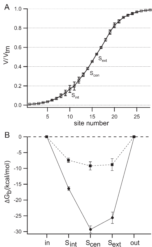
Figure 6. Chloride binding and movement in the pore. (A) The CIC-0 homology models created as described in Materials and methods were used to calculate the electrostatic potential at various positions in the pore ( V/V_{tm} ) under an externally applied transmembrane voltage of -200 mV. Shown here is the fraction of the transmembrane voltage along a hypothetical permeation pathway, with S_{int} , S_{cen} , S_{ext} at sites 10, 14, and 16, respectively. (B) The CIC-0 homology model was used to calculate the electrostatic contribution to the free energy of chloride binding ( \Delta G_b ) to each site in the pore (starting from the cytoplasmic side: S_{int} , S_{cen} , S_{ext} ) with either zero (circles) or two (squares) chlorides already bound in the pore. The dielectric constant used for the protein was 4. In both A and B, lines connect data points for ease in viewing, and error bars represent an estimate of the discretization error arising from the grid-based Poisson-Boltzmann calculations (see Materials and methods).
