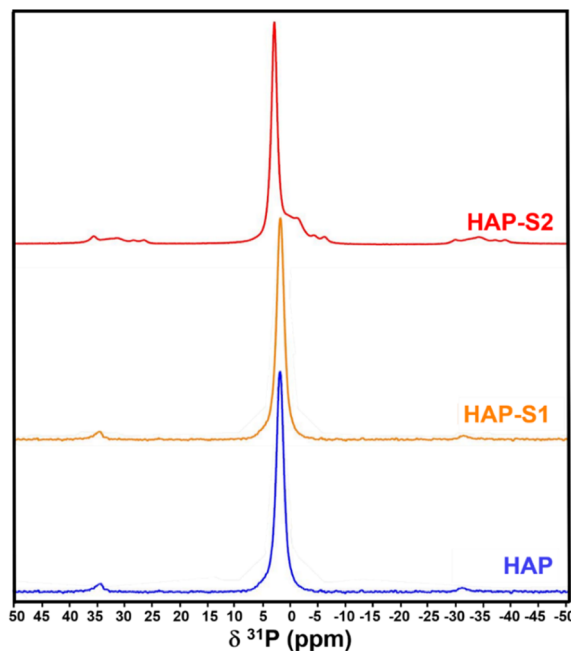
Fig. 4 ^{31}\text{P} -MAS-NMR spectra of the prepared samples.
