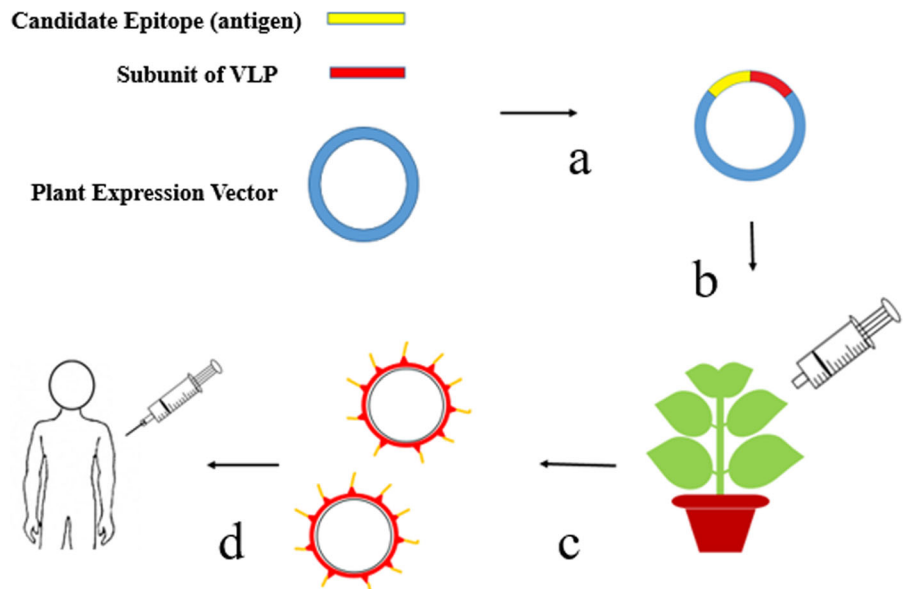
Fig. 1 Schematic review of recombinant protein expression in plants. VLP Virus-like particle, a Recombinant vector construction, b Agroinfiltration in plants, c 3–7 days post-infiltration recombinant proteins are expressed in the leaves, and VLP subunits assembled into VLPs displaying epitope on the surface, and d VLPs are purified and used as a vaccine to induce immune responses
