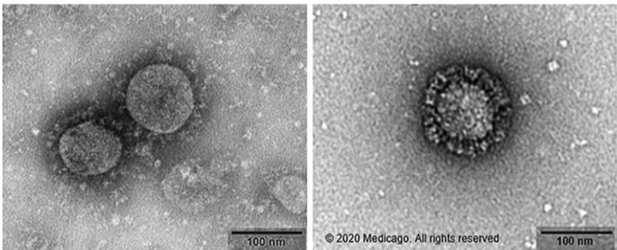
Fig. 2 Comparison of SARS-CoV-2 VLP made by Medicago with wild-type SARS-CoV-2 (Ward et al., 2021) https://www.medicago.com/en/ . SARS-CoV-2 Severe acute respiratory
