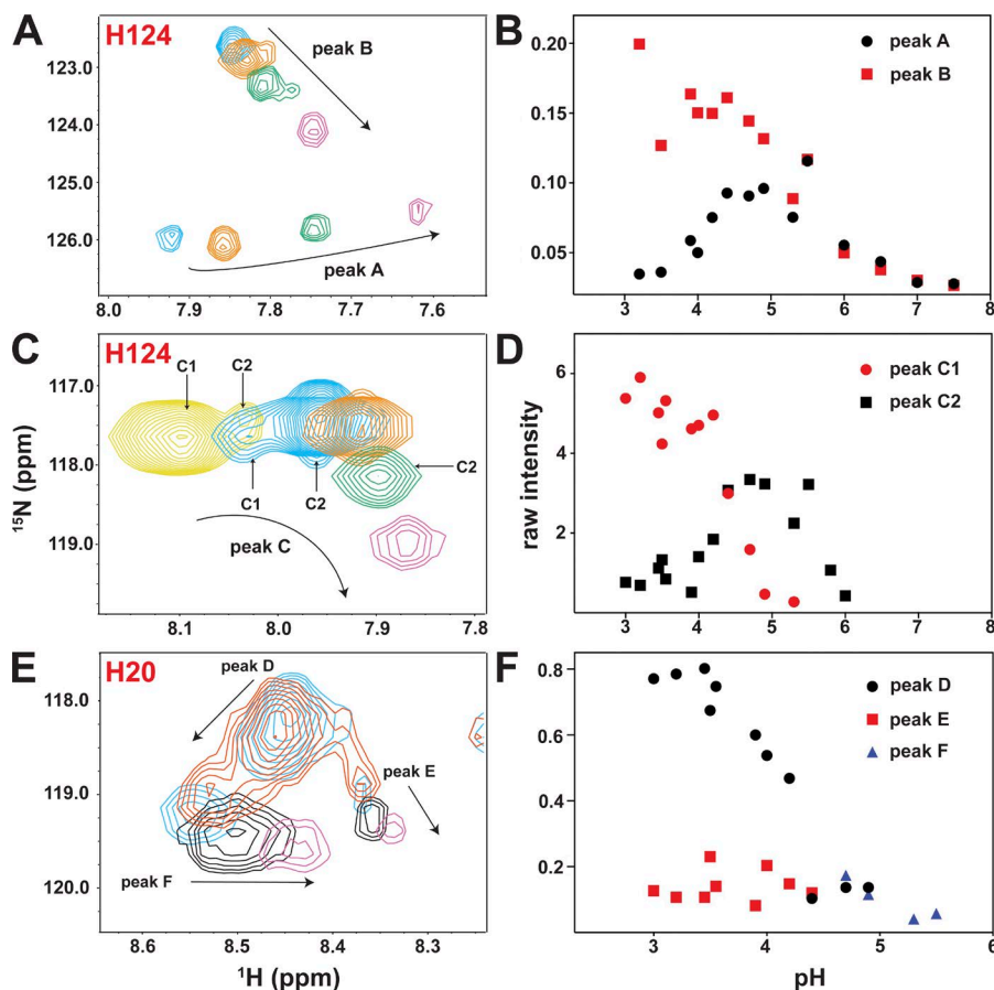
Figure 3. Histidine peaks change with pH in the [^1\text{H},^{15}\text{N}] HSQC spectrum of WT KcsA \Delta\text{C} . (A) pH-dependent chemical shift changes of the C-terminal H124 peaks (labeled peaks A and B) at pH 4.5 (blue), 5.5 (orange), 6.5 (green), and 7.5 (pink). Peaks A and B are observed through the pH range measured (pH 3–8). (B) Raw intensities plotted for C-terminal H124 peaks A and B as a function of pH. (C) pH-dependent chemical shift changes of the primary H124 peaks (labeled C1 and C2) at pH 3.0 (yellow), 4.5 (blue), 5.5 (orange), 6.5 (green), and 7.5 (pink). C1 and C2 peaks are marked with an arrow for pH 3.0 and 4.5. At pH 5.5, 6.5, and 7.5 only C2 is visible. (D) Raw intensities plotted for primary H124 peaks C1 and C2 as a function of pH. (E) pH-dependent chemical shift changes of the H20 peaks (labeled peaks D–F) at pH 3.7 (red), 4.0 (blue), 5.0 (black), and 5.5 (pink) showing their pH-dependent changes in chemical shift. (F) Raw intensities plotted for H20 peaks D–F.
