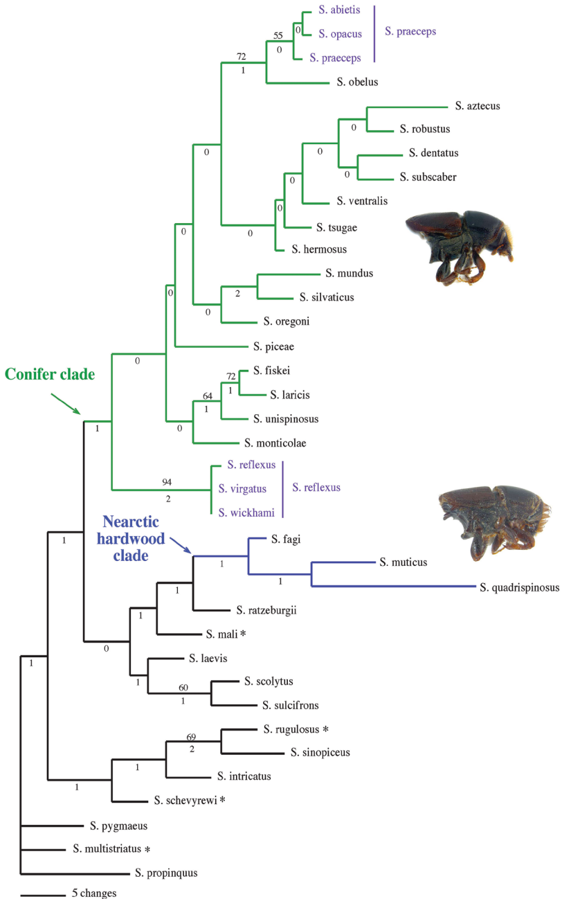
Figure 2. Morphological phylogeny of Nearctic Scolytus . Phylogram of one of 1016 most parsimonious trees (L = 262, CI = 0.332, RI = 0.539) generated for 37 taxa with 43 characters from a heuristic search of 1000 stepwise random additions with TBR in PAUP*. Numbers above the node indicate bootstrap values (>50). Bremer support values are listed below the node. The Nearctic hardwood and conifer clades are indicated in blue and green respectively. Non-monophyletic species are indicated in purple. * denotes species exotic to the Nearctic.
