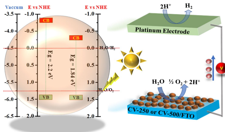
Figure 8. Band edge positions and PEC water splitting mechanism of CV-250 and CV-500.
