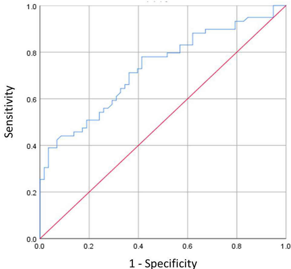
Figure 1 The ROC curve of the rheumatoid factor levels for dry eye with common autoimmune diseases. The AUC of the ROC curve for rheumatoid factor was estimated to be 0.73 (95% confidence interval [CI]: 0.639–0.821, P < 0.001 ).
