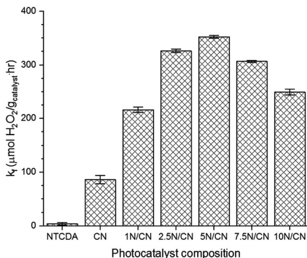
Fig. 5 Comparison of the rate of photochemical formation of H 2 O 2 by NTCDA/CN heterojunctions. Control samples of pure CN and pure NTCDA are also presented for comparison. Error bars represent the standard error of the mean (SEM) of two unique trials.
