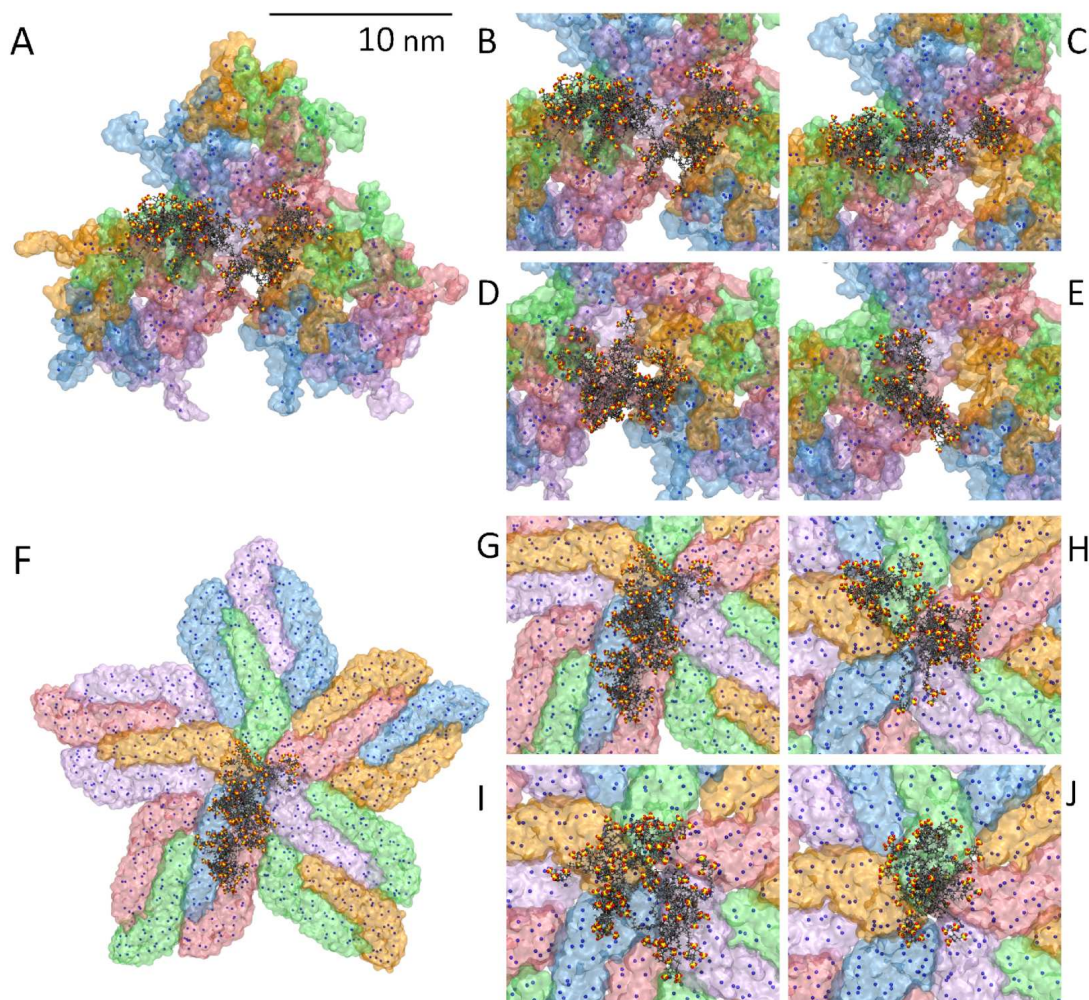
FIG. 7. (A) Binding of L8E to HPV capsid L1 proteins. (B-E) Detailed views for L8E, LG1E, C5E and TG1E, respectively. (F) Binding of L8E to dengue virus E proteins. (G-J) Detailed views for L8E, LG1E, C5E and TG1E, respectively. The dots show the positions of positive charges on the protein surfaces.
