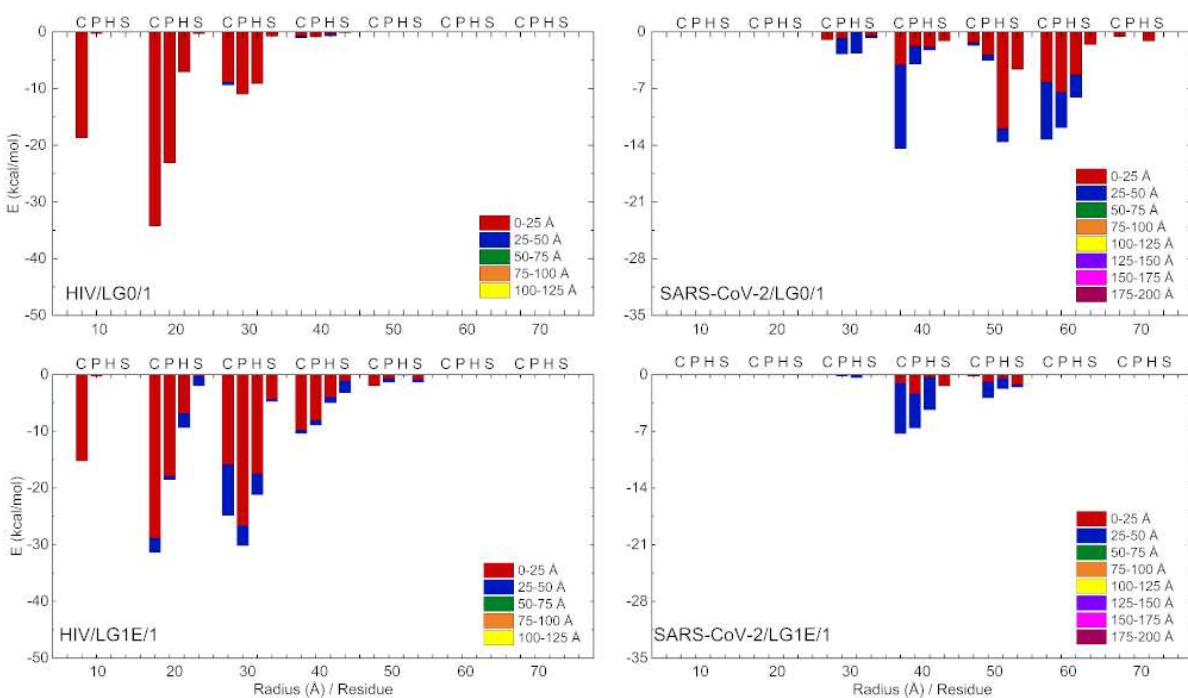
FIG. 5. Dominant residue-resolved drug-receptor binding energies between LG0/LG1E mimics and HIV/SARS-CoV-2 protein receptor trimers (Fig.2). The energies are calculated by VMD (without implementing PME to account for the presence of screening), and averaged over the last 20 ns of simulations. The x-axis shows the distance of the residue from the symmetry axis of the gp120 trimer, while different colors show the vertical distance of the residue from the top of the trimer. The protein complex was divided into cylindrical shells of radii growing by 1 nm and height of 2.5 nm. The presence of selected residues in these cylindrical shells provide selected contributions to the binding energies. The residues are grouped according to their types: charged (C): ARG, HSD, LYS, ASP, GLU; polar (P): SER, THR, ASN, GLN; hydrophobic (H): ALA, VAL, ILE, LEU, MET, PHE, TYR, TRP; special (S): CYS, GLY, PRO.
