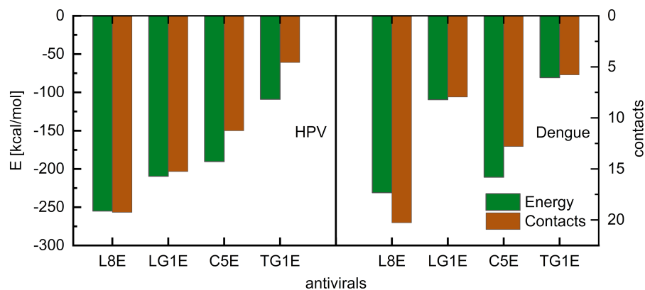
FIG. 8. Direct binding energies and numbers of basic contacts obtained between sulfonated drugs and surface protein assemblies in HPV and dengue viruses. PME was disabled in the energy calculations (see Methods). Basic residues were counted when they were closer than 4 Å to the drugs.
