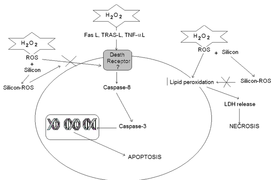
Figure 7 Diagram of the mechanism by which both H_2O_2 and Si induce cellular damage and neuroprotection. H_2O_2 inducing apoptosis: H_2O_2 , perhaps, by induction of death ligand, may activate death receptor responsible to activate caspase-8 (inductor enzyme) which activates caspase-3 (effectors enzyme). This last enzyme damages DNA and protein and as consequence produces apoptosis. H_2O_2 inducing necrosis: H_2O_2 (ROS) induces lipid peroxidation which conduces to LDH release and necrosis death. Si effect: In the presence of Si, H_2O_2 treated cells remove H_2O_2 (ROS) preventing neurotoxicity induced by it.
