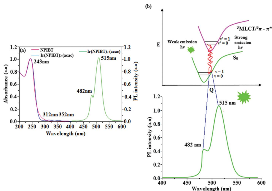
Fig. 5 (a) UV and PL spectra of NPIBT and Ir(NPIBT) 2 (acac); (b) representative Franck–Cordon electronic transitions of Ir(NPIBT) 2 (acac).
