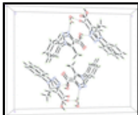
Fig. 2. A view of the packing of the title compound, stacking along the a axis.
