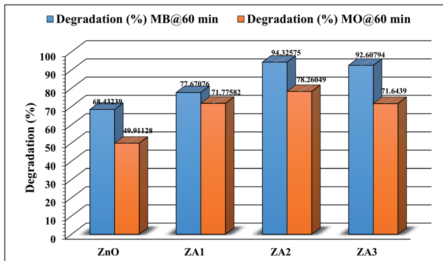
Fig. 6 Photocatalytic degradation of MB and MO over ZnO and ZnO/Alg bionanocomposite (dye concentration = 20 mg L -1 , catalyst dosage = 20 mg, irradiation time = 60 min).
