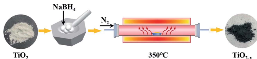
Fig. 1 Schematic diagram of the typical \text{TiO}_{2-x} preparation process.
