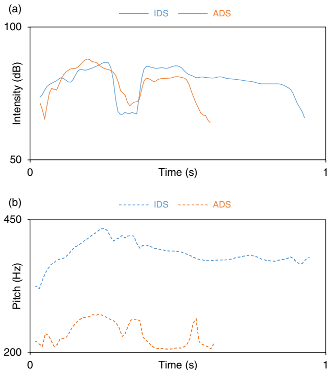
FIGURE 2 Intensity (a) and pitch (b) of the two speech samples used in the IDS and ADS conditions. The two samples had identical mean intensity and similar intensity profiles. Consistently with IDS characteristics in other languages, the two Lenakel utterances used in the experiment differed in pitch ( \text{mean}_{\text{IDS}} = 387 \text{ Hz} , \text{mean}_{\text{ADS}} = 235 \text{ Hz} ), pitch range ( \text{max}_{\text{IDS}} - \text{min}_{\text{IDS}} = 114 \text{ Hz} , \text{max}_{\text{ADS}} - \text{min}_{\text{ADS}} = 65 \text{ Hz} ) and duration, resulting mostly from the elongation of the last vowel in the IDS utterance (IDS: 0.96 s, ADS: 0.64 s)
