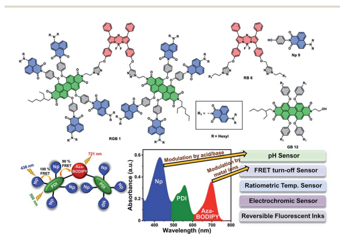
Fig. 1 Chemical structures of RGB antenna 1 , RB 6 and GB 12 , and Np 9 and schematic representation of the RGB antenna for multiparameter sensing.
