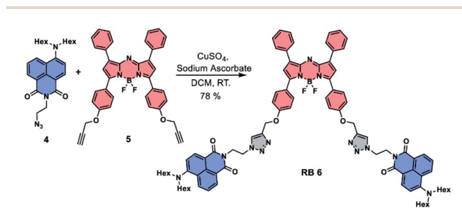
Scheme 1 Synthesis of RB antenna 6 .
