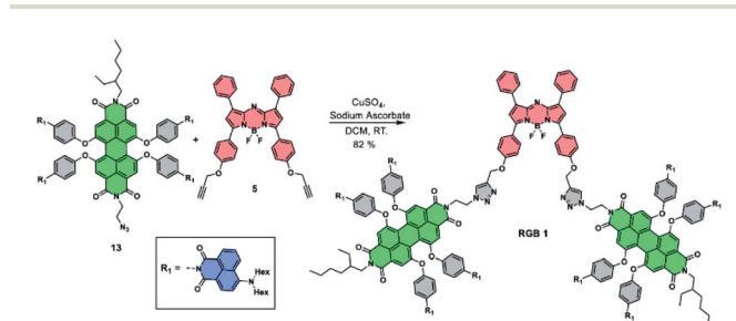
Scheme 2 Synthesis of RGB antenna 1 .
