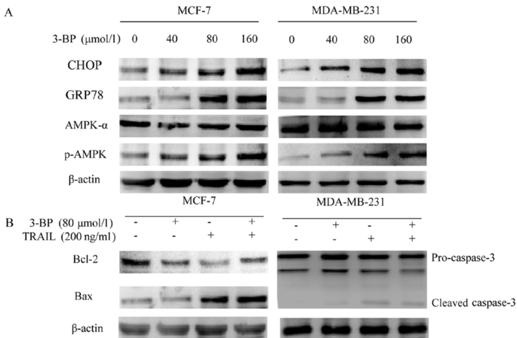
Figure 3. 3-BP induces AMPK phosphorylation and induces cell death. (A) The levels of CHOP, GRP78, AMPK-α and p-AMPK were detected in breast cancer MCF-7 and MDA-MB-231 cells treated with 3-BP (0, 40, 80 and 160 μmol/l) for 24 h via western blot analysis. (B) The expression levels of Bax in MCF-7 cells and caspase-3 protein in MDA-MB-231 cells were detected via western blotting in cells treated with 80 μmol/l 3-BP and 200 ng/ml TRAIL. 3-BP, 3-bomopyruvate.
