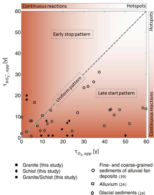
Fig. 3. Apparent O_2 versus apparent NO_3^- reaction times determined from field data for different aquifer types. The comparison provides information on the vertical pattern of reactivity (late start and early stop pattern) and related stratum reaction times. The dark brown color in the background indicates continuous reactions within the reactive stratum with short reaction times, and the light brown background indicates hot spots within the reactive stratum with larger reaction times depending on the density of hot spots ( Materials and Methods and SI Appendix, section S2 ). The dominance of the late start pattern in aquifers is noticeable, with 79% of the data points indicating that reactions occur after a nonreactive time lag.
