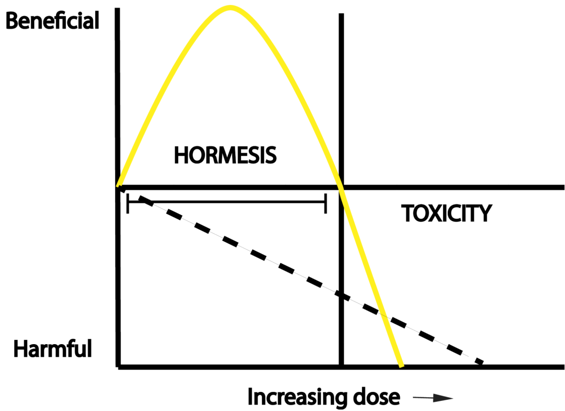
Figure 3. Concept of ROS hormesis
