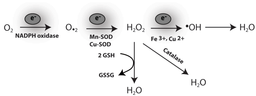
Figure 1. Biochemistry of ROS
