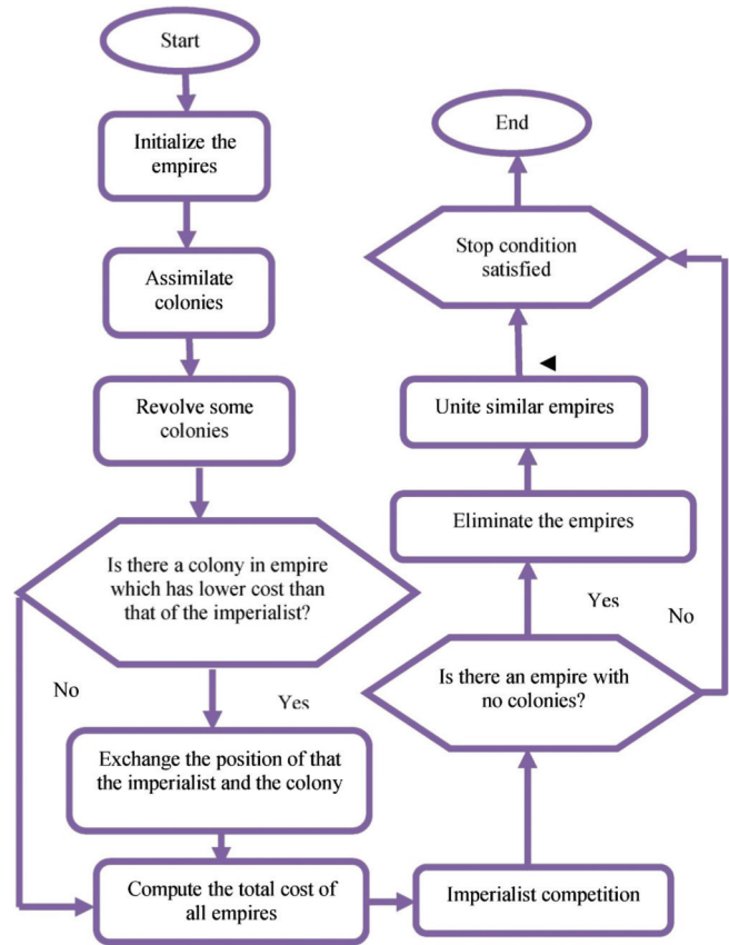
Figure 1: Imperialist competitive algorithm flowchart [58]
