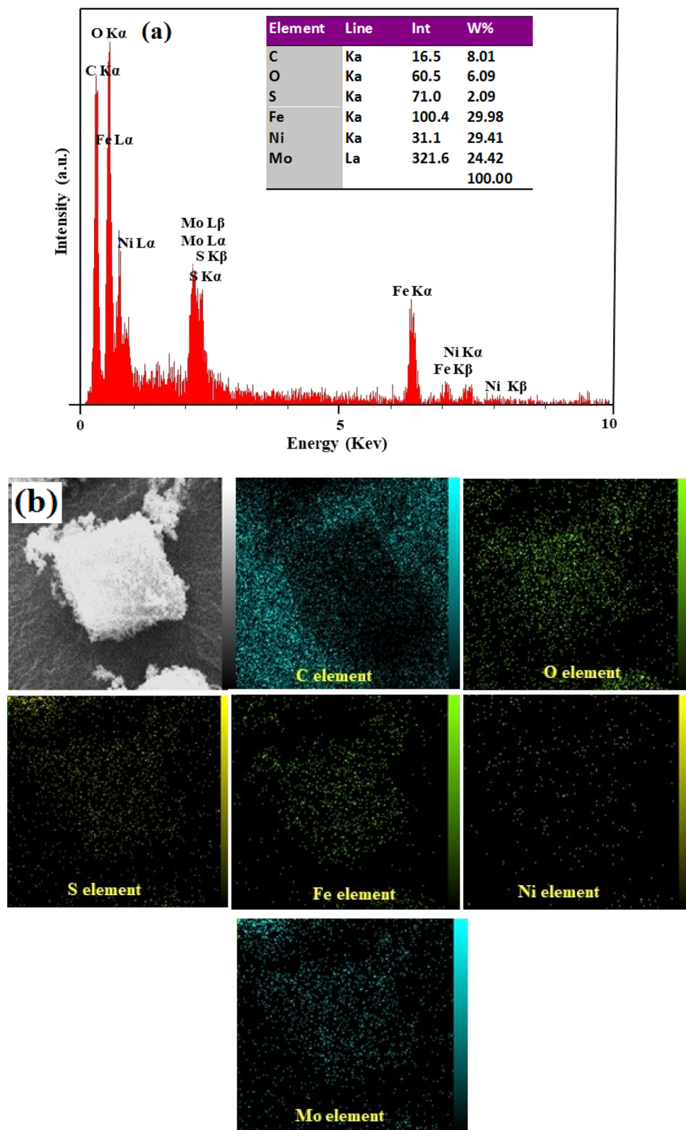
Fig. 5 (a) EDX spectrum and (b) an indicative SEM image of the MoS 2 /NiFe 2 O 4 /MIL-101(Fe) with corresponding elemental mappings.
