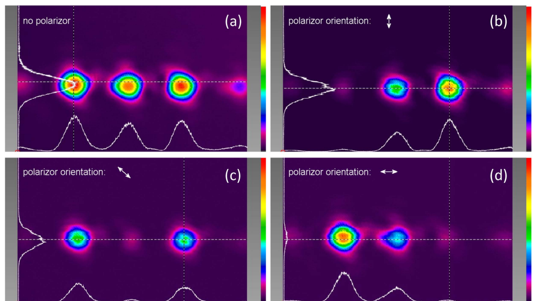
Figure 6. Far-field intensity distribution in the back focal plane of lens L7. (a) With no polarizer in front of the camera; (b) when the polarizer is aligned vertically in front of the camera; (c) when the polarizer is oriented at 135 degrees in front of the camera; (d) when the polarizer is aligned horizontally in front of the camera.
