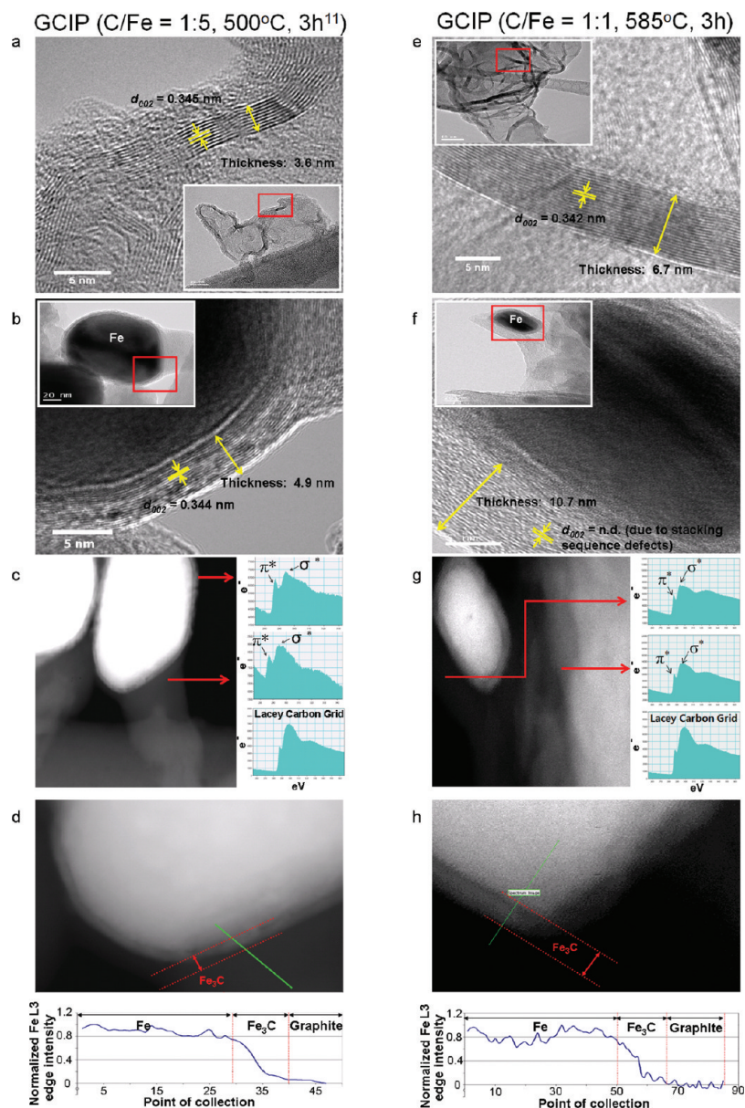
Figure 5. Comparison of HRTEM measurements of the AMS target of GCIP 11 and the AMS target of GCIP (C/Fe = 1:1, 585 °C, 3 h). Both AMS targets of GCIP consisted of carbon (/or graphite) sheet (a and e) and the carbon-encapsulated Fe (C-Fe, b and f). Enlarged images of the carbon sheet (a and e) and the C-Fe (b and f) matched the red rectangle area in each insert TEM image. The carbon sheet in the AMS target of GCIP (C/Fe = 1:1, 585 °C, 3 h) was more ordered ( d_{002} = 0.342 nm) and thicker (6.7 nm) than that of the AMS target of GCIP 11 (a and e). The carbon shell in the AMS target of GCIP (C/Fe = 1:1, 585 °C, 3 h) was thicker (10.7 nm) than that in the AMS target of GCIP 11 (4.9 nm). However, the carbon shell in the AMS target of GCIP (C/Fe = 1:1, 585 °C, 3 h) was a less ordered carbon (b and f) compared to that in the AMS target of GCIP. 11 Although all graphitization processes were conducted under identical conditions, carbon shell thickness in the AMS target of GCIP was variable, because our Fe particle size was not uniform. STEM-EELS showed ordered, semioordered, and amorphous carbons in both AMS targets of GCIP. The EELS of both AMS targets of GCIP were consistent for those of graphite and a-C in a prior study 28 (c and g). The STEM-EELS line scan was performed to check the Fe composition along the C-Fe interface, along the green line (d and h). The distance between each spectrum was about 0.3 nm, and it was normalized to the FeL3 intensity along the green line. Even though the Fe 3 C in the C-Fe was not uniform, it was detected by \approx 5 nm deep into the Fe particle.
