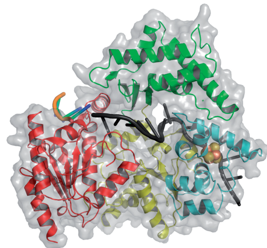
Figure 3. Structure of the T. acidophilum XPD-DNA complex. Overall structure of XPD, shown in a transparent surface representation, with the two RecA-like domains in yellow and red, the FeS cluster domain in cyan, and the arch domain in green. The 4Fe-4S cluster is shown by the spheres with orange (Fe atom) and yellow (Cys residue) colors. The DNA identified in the electron density is shown in orange. Combination of experimentally verified DNA is shown in orange with modeled DNA shown in gray. Figure was provided by Drs Jochen Kuper and Caroline Kisker (45).
