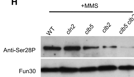
Figure 1. Analysis of Fun30-S28 phosphorylation in cell cycle and in response to DNA damage. (A) Alignment of the N-terminal amino acid sequences for Fun30 and its orthologs from indicated species. The evolutionarily conserved serine is marked with an asterisk. (B) Western blot analysis of Fun30-S28 phosphorylation in wild type cells and FUN30 mutants. All FUN30 alleles were fused C-terminally to a sequence encoding 13xMYC. (C) Western blot analysis of Fun30-S28 phosphorylation in cells arrested in different phases of the cell cycle. (D) In vitro phosphorylation of Fun30 and fun30-3A by the Cdk1-Clb2 complex. (E) Western blot analysis of Fun30-S28 phosphorylation in wild type cells with or without drug treatments. (F) Western blot showing Rad53 phosphorylation upon MMS treatment in the wild type strain and indicated mutants. (G,H) Western blot showing Fun30-S28 phosphorylation in wild type cells and indicated mutants upon MMS treatment.
