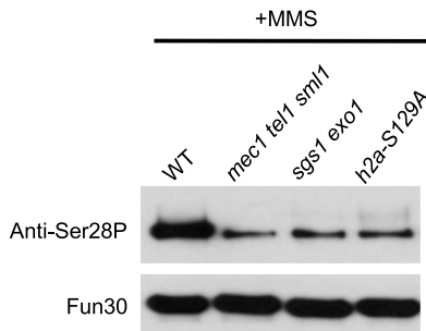
Figure 1. Analysis of Fun30-S28 phosphorylation in cell cycle and in response to DNA damage. (A) Alignment of the N-terminal amino acid sequences for Fun30 and its orthologs from indicated species. The evolutionarily conserved serine is marked with an asterisk. (B) Western blot analysis of Fun30-S28 phosphorylation in wild type cells and FUN30 mutants. All FUN30 alleles were fused C-terminally to a sequence encoding 13xMYC. (C) Western blot analysis of Fun30-S28 phosphorylation in cells arrested in different phases of the cell cycle. (D) In vitro phosphorylation of Fun30 and fun30-3A by the Cdk1-Clb2 complex. (E) Western blot analysis of Fun30-S28 phosphorylation in wild type cells with or without drug treatments. (F) Western blot showing Rad53 phosphorylation upon MMS treatment in the wild type strain and indicated mutants. (G,H) Western blot showing Fun30-S28 phosphorylation in wild type cells and indicated mutants upon MMS treatment.
