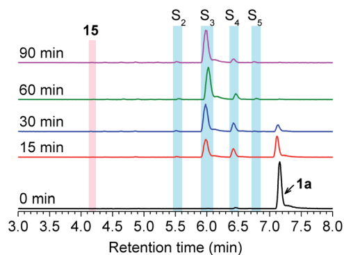
Fig. 5 UPLC-MS chromatograms of RSSH generation from 1a ( 100 \mu M ) in the presence of lysine ( 500 \mu M ) in pH 7.4 ammonium bicarbonate ( 50 \text{ mM} ) containing the metal chelator DTPA ( 100 \mu M ) at 37^\circ C . Aliquots taken at various times were quenched with 1% formic acid and analyzed by UPLC-MS. RSSH-derived symmetrical dialkyl polysulfide, labeled as S_2 to S_5 ( R^1SS_nSR^1 , n = 0-3 , cyan highlight), formation is evident. The very minor peak at 4.17 \text{ min} corresponds to carbamate 15 .
